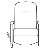
PRRT-13, Treatment Chair W-34½", D-36", H-47½", SH-19", AH-25½" Fully reclined-76"
