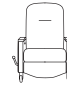
PRRT-12, Treatment Chair W-34½", D-36", H-47½", SH-19", AH-25½" Fully reclined-76"
