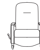
PRRT-12, Treatment Chair, with optional fold-down arm W-34½", D-36", H-47½", SH-19", AH-25½" Fully reclined-76"
